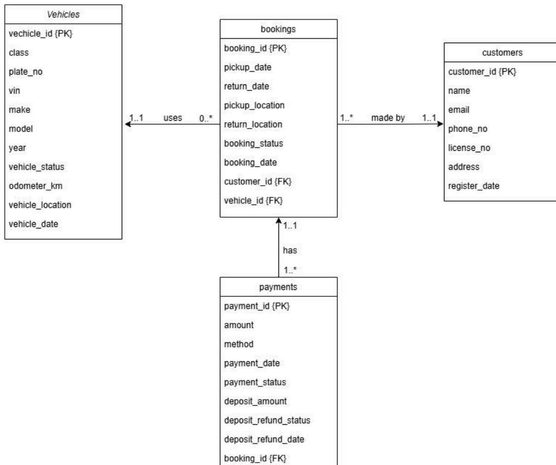
Figure 1.0 ERD of Car Rental System
